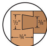
LARGE DRAWER BACK SIDE DOVETAILS
