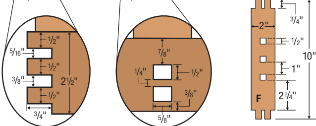
DRAWER DIVIDER
