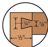
MEDIUM/SMALL DRAWER BACK SIDE DOVETAILS
