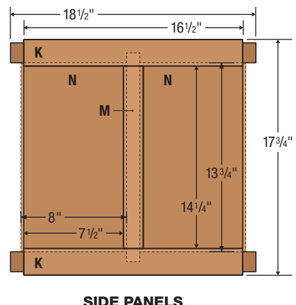
SIDE PANELS
