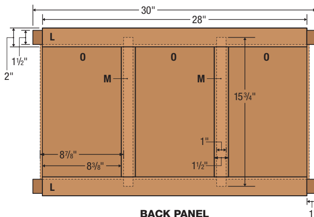
BACK PANEL
