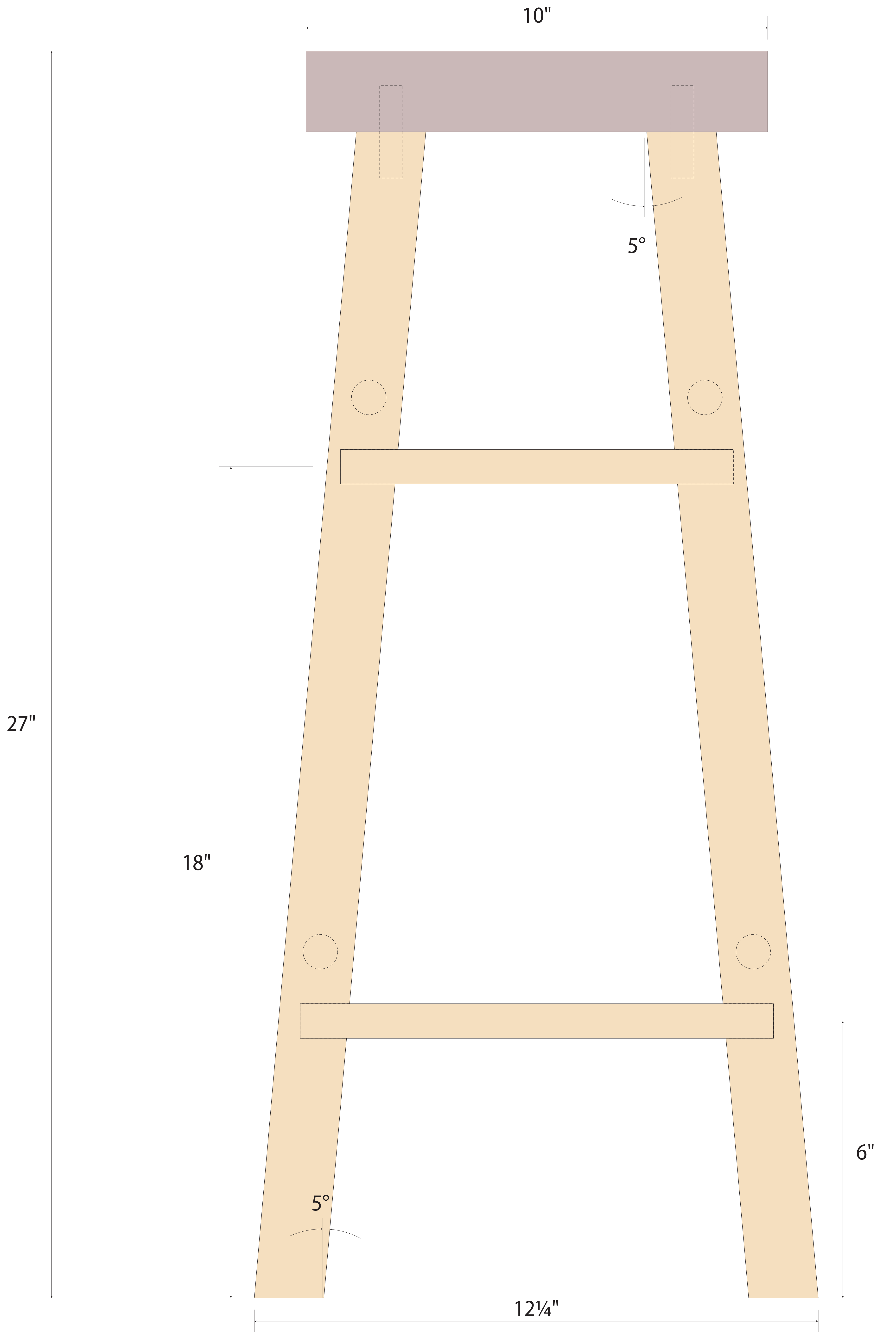
Kitchen Stool Side
