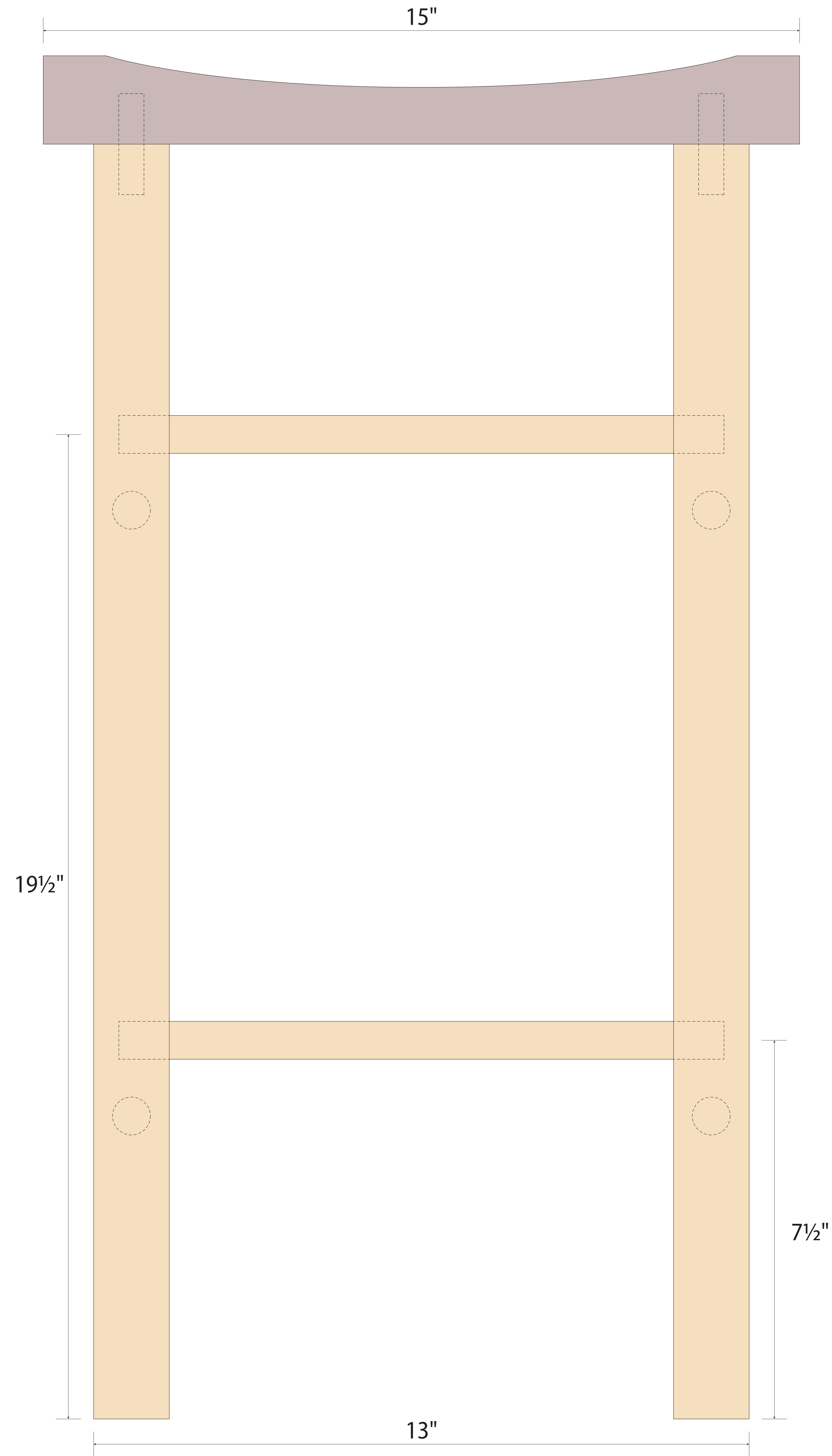
Kitchen Stool Front
